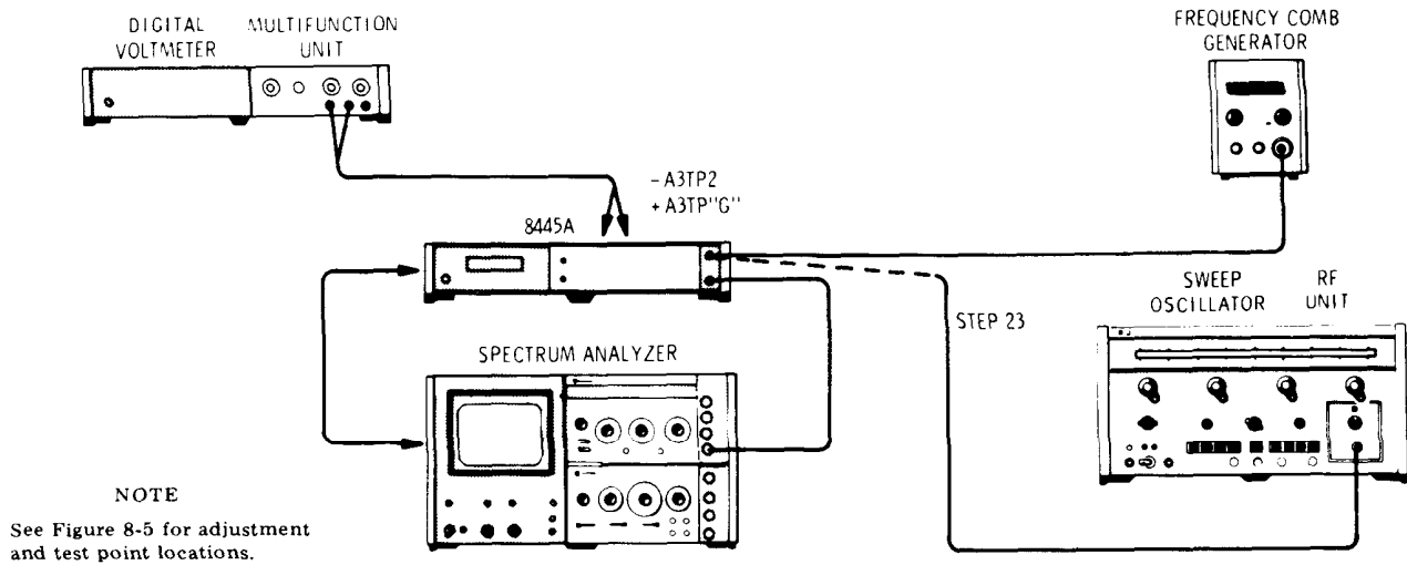
Figure 5-4. Yig Driver Check and Adjustment Test Setup (Matched Operation)
