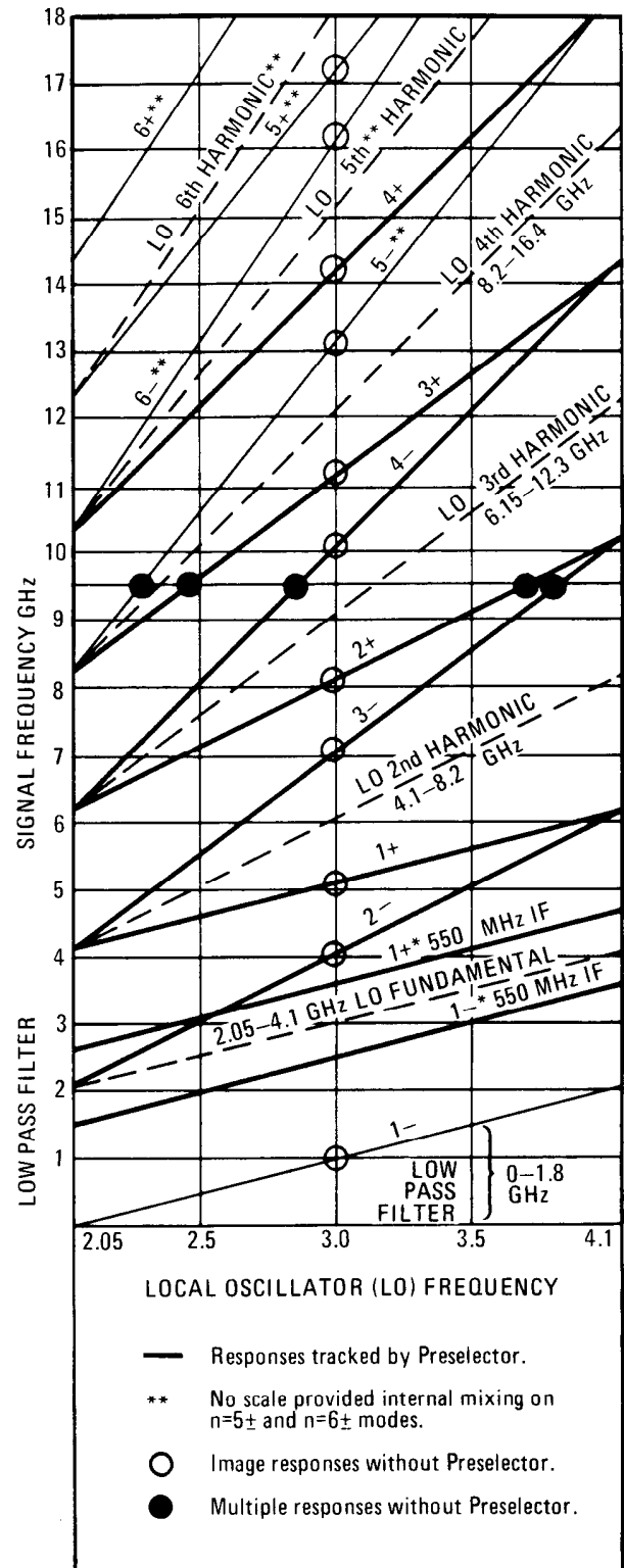
Figure 3-7. Spectrum Analyzer Tuning Curves and Responses
