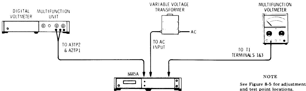
Figure 5-1. Power Supply Check and Adjustment Test Setup
