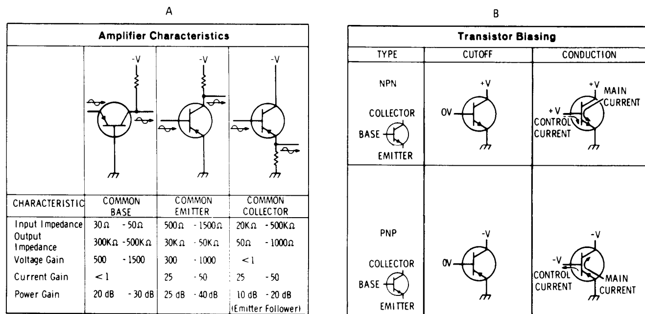
Figure 8-1. Transistor Operation
